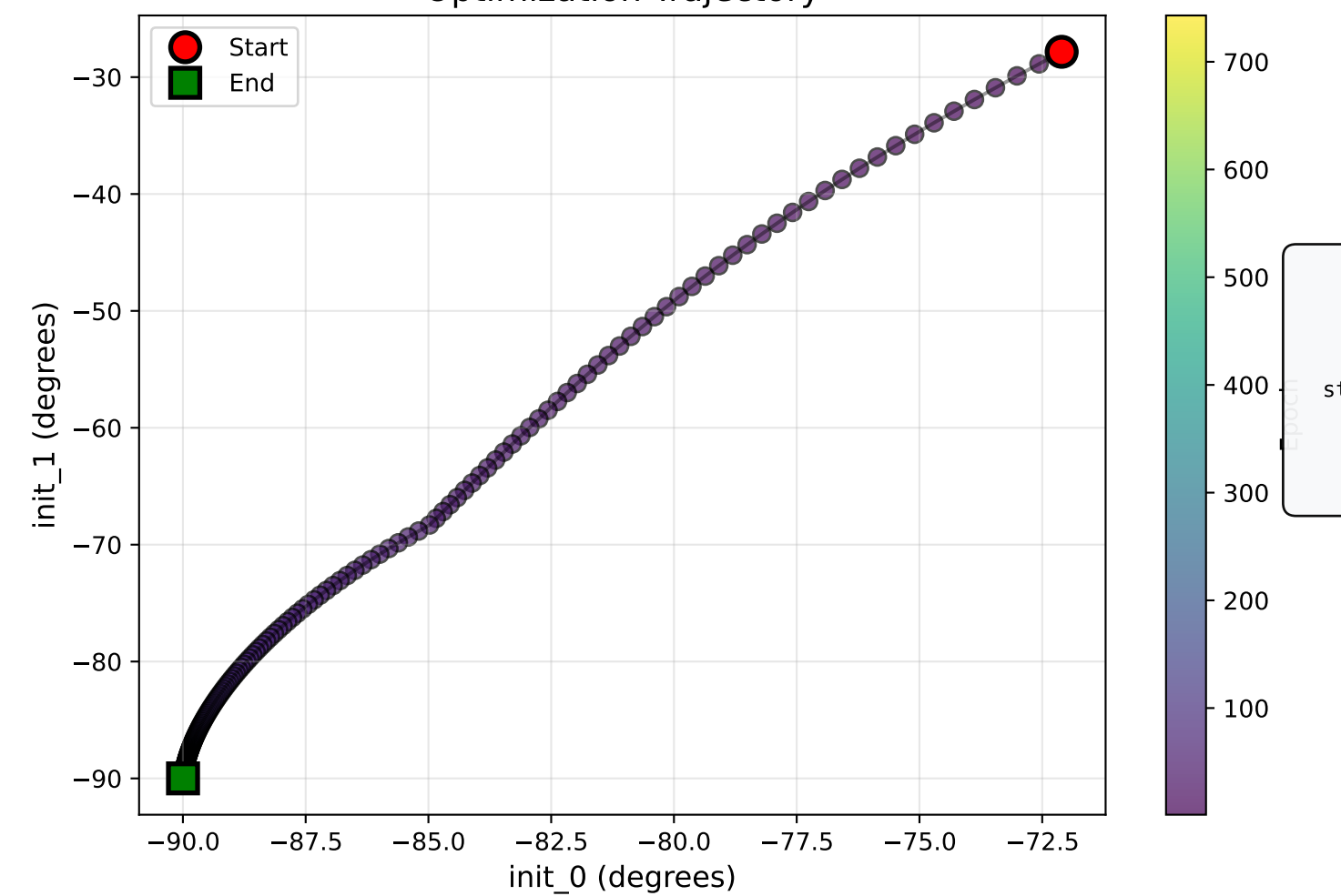
Optimization Trajectory
